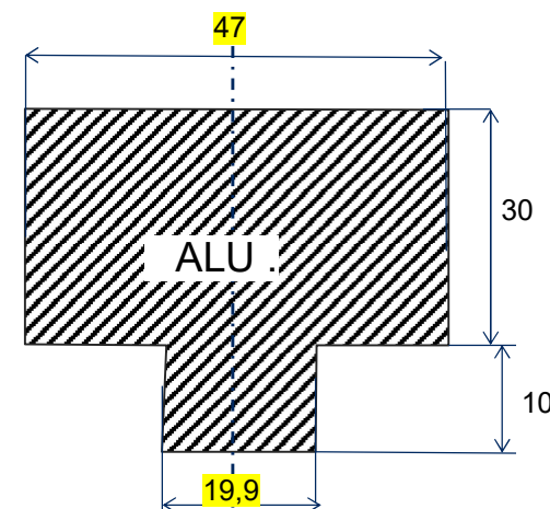
Embout insertion 20
