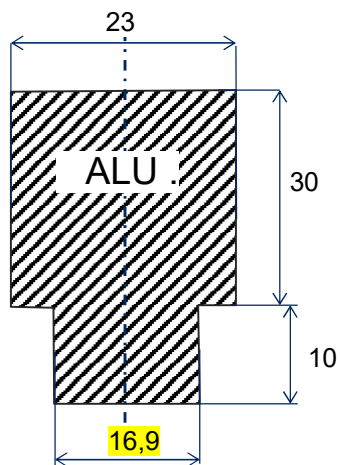
Embout extraction 17
