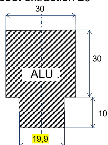
Embout extraction 20
