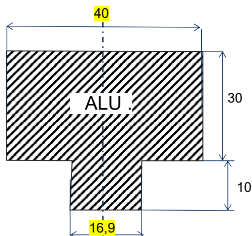
Embout insertion 17
