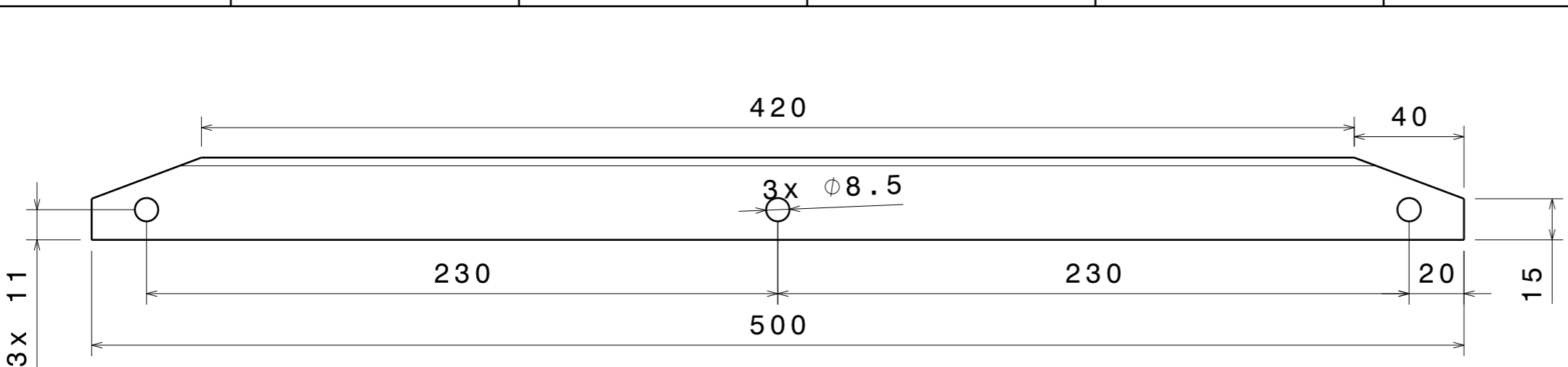
Front view Scale : 1:2
