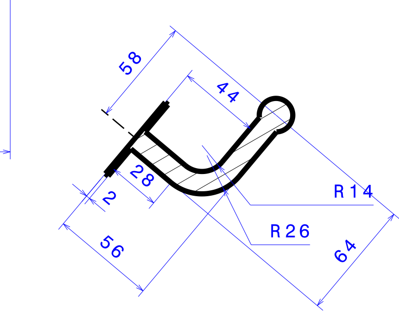
Section view C-C Scale: 1:2
