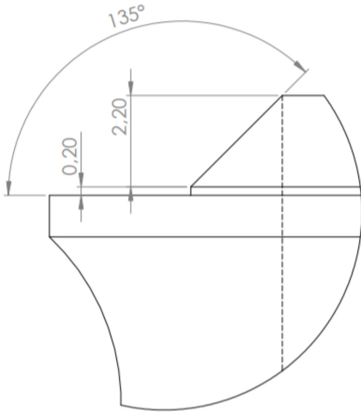
DETAIL A SCALE 10 : 1
