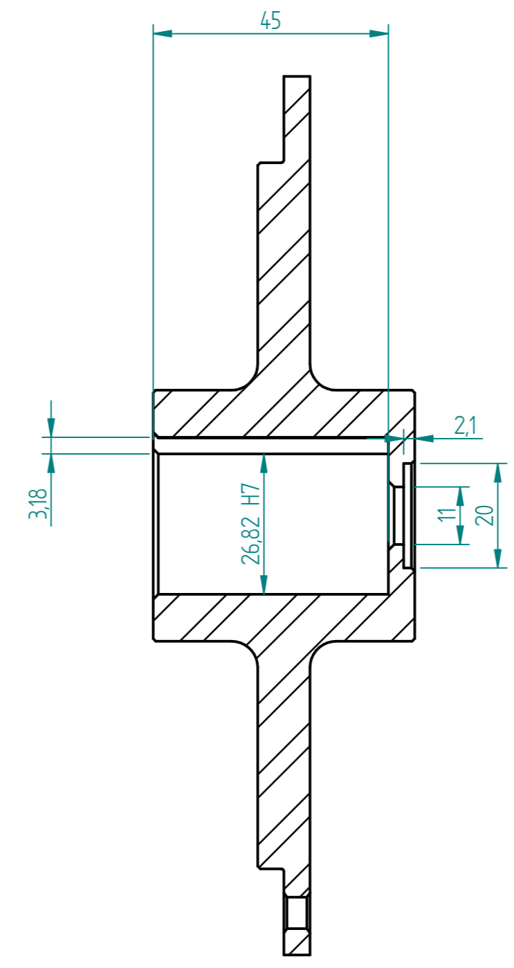
SECTION B-B
