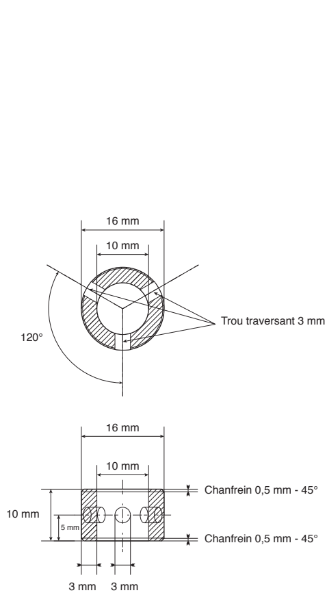
6 Bagues acier standard
