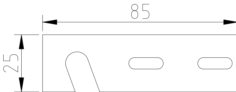
wheelMount.dxf (x8 alu 4mm)
