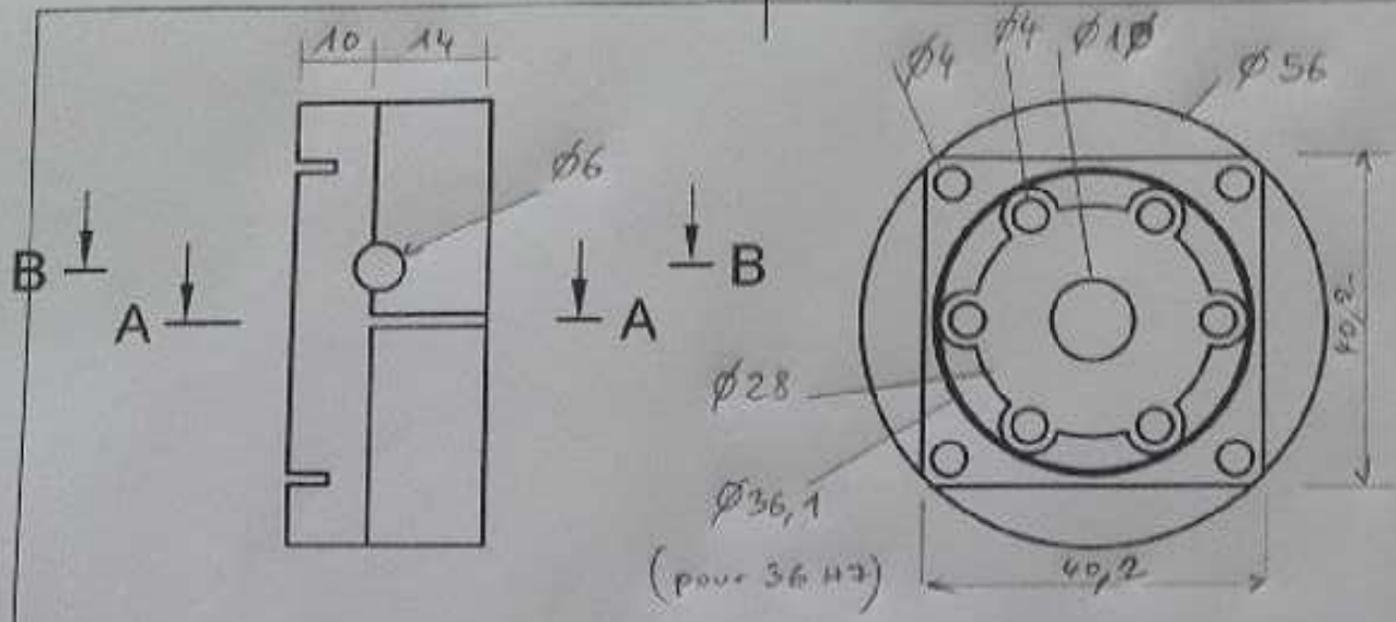
B-B (1:1)
