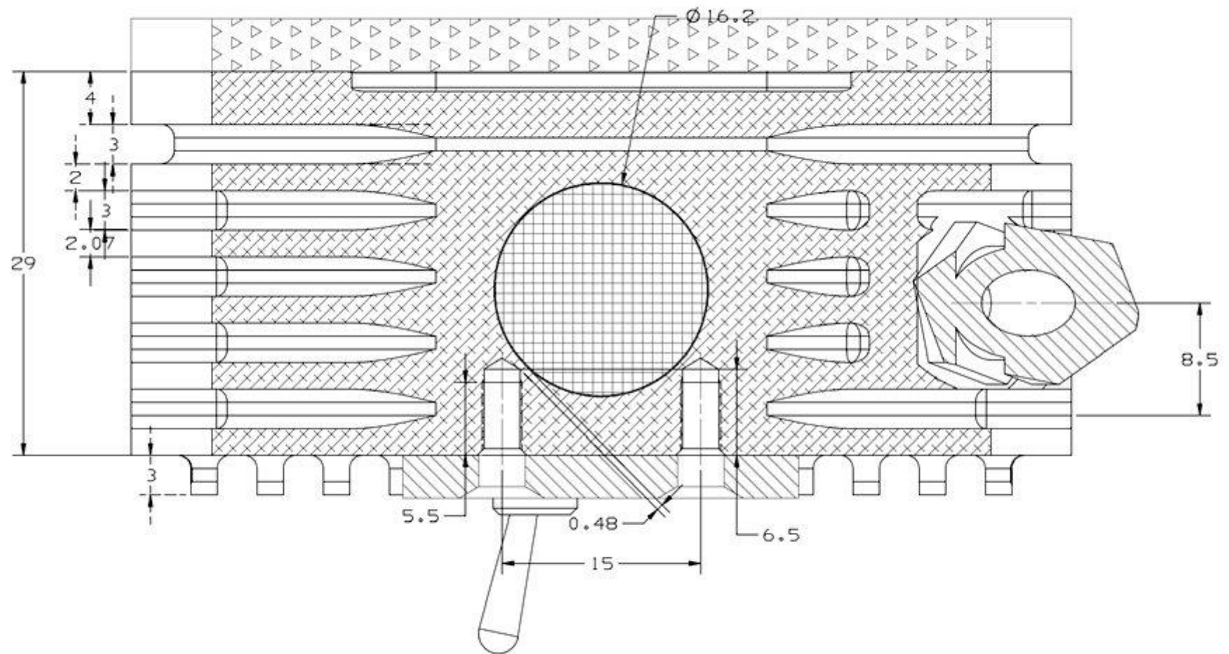
SECTION A - A SCALE 4:1
