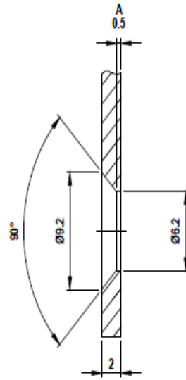
DETAIL -C- SCALE 3:1
